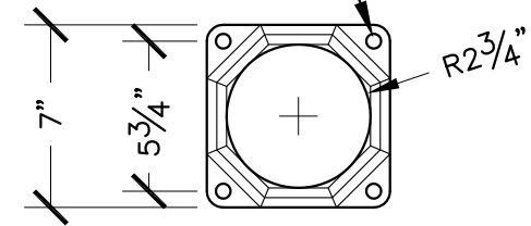
BASE ANCHORAGE
